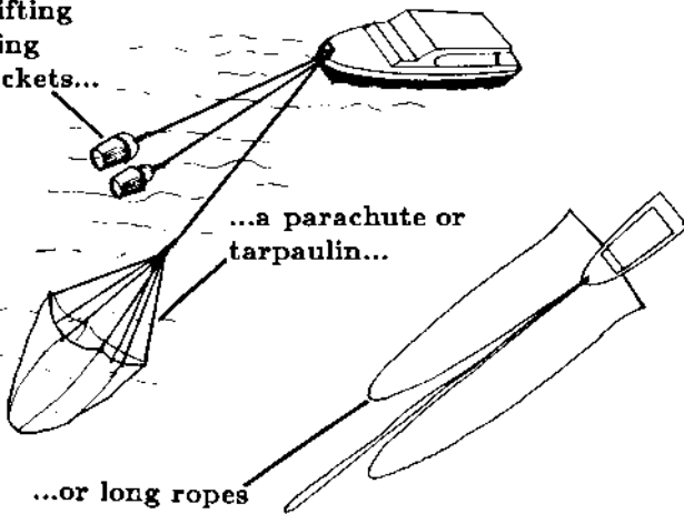
Anchors and sea anchors
