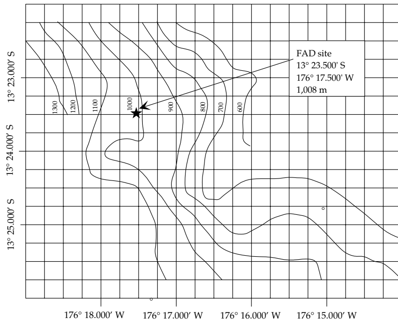
Figure 5: Bottom contour map and FAD site selected in the Passe Honikulu survey zone
