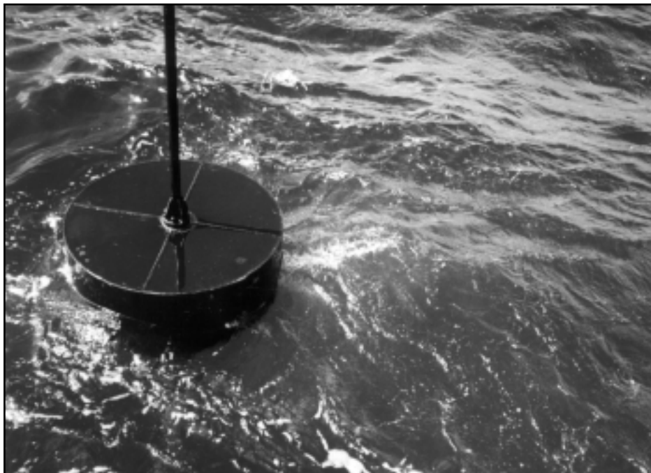
Figure 15: Spar buoy released at the completion of deploying the Wallis FAD anchor first
